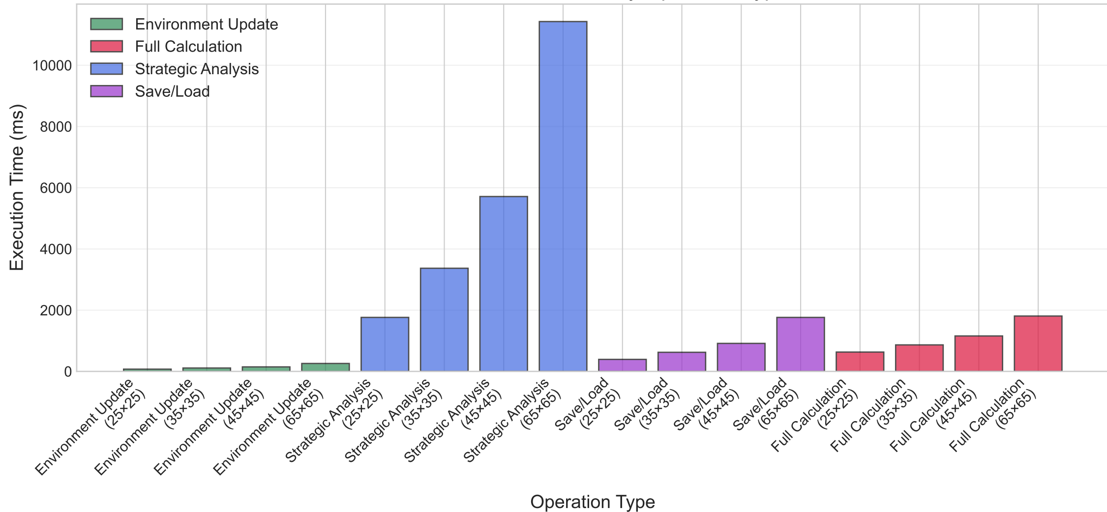
Performance Overview by Operation Type
